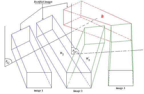
Fig. 1. Rectification principle for a triplet of images.
